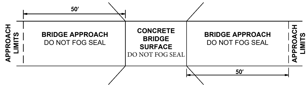
DETAIL FOR MAP # 1 / STRUCTURE # 0332
